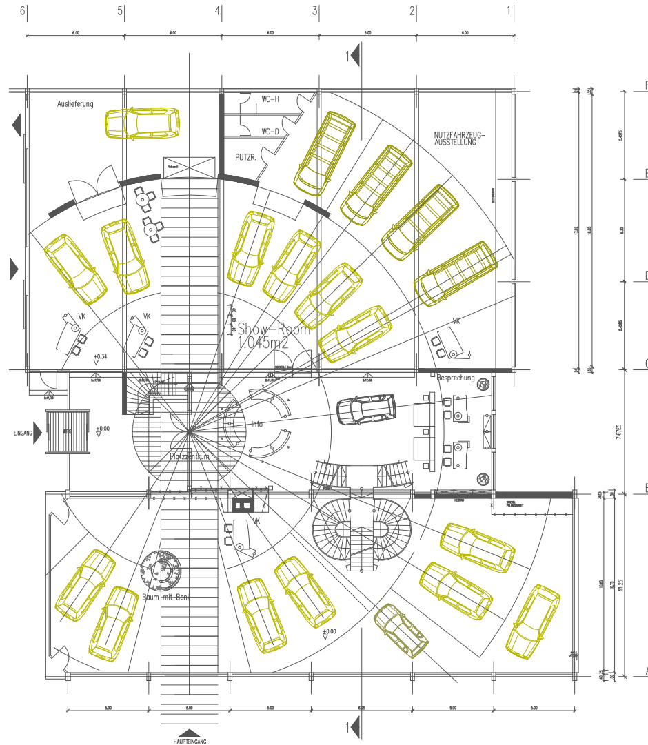
SHOWROOM GRUNDRISS
